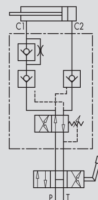
SCHEMA IDRAULICO HYDRAULIC DIAGRAM
